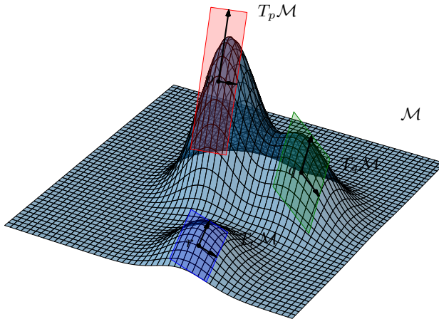
Figure 20: Tangent spaces at points p , q , and r in an arbitrary manifold \mathcal{M} . The arrows are the respective basis vectors on the embedding axes.
